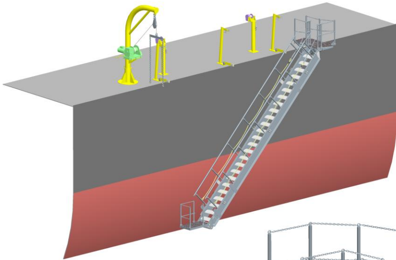
Deployed
