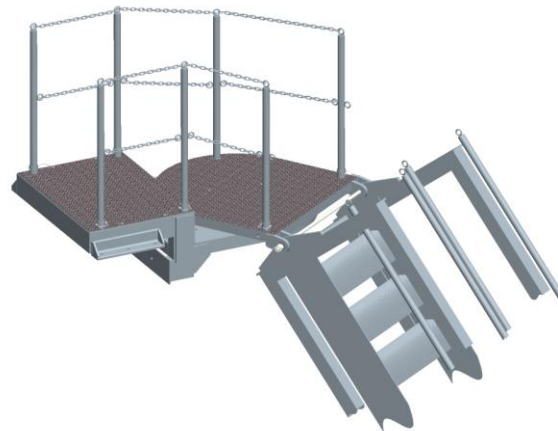
Rotating Platform
