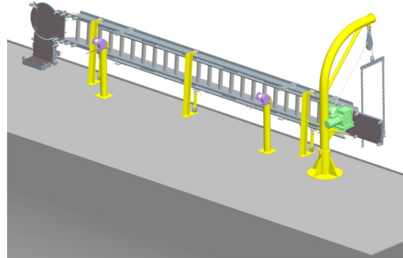
Stowed
