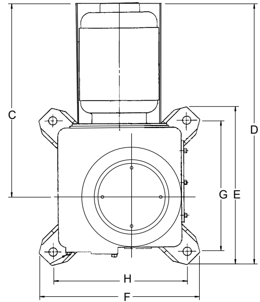
Pull-Pak 100A
